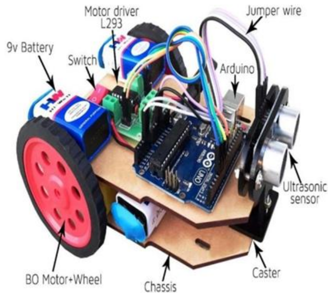
Fig. 4: Side View of the Robot
