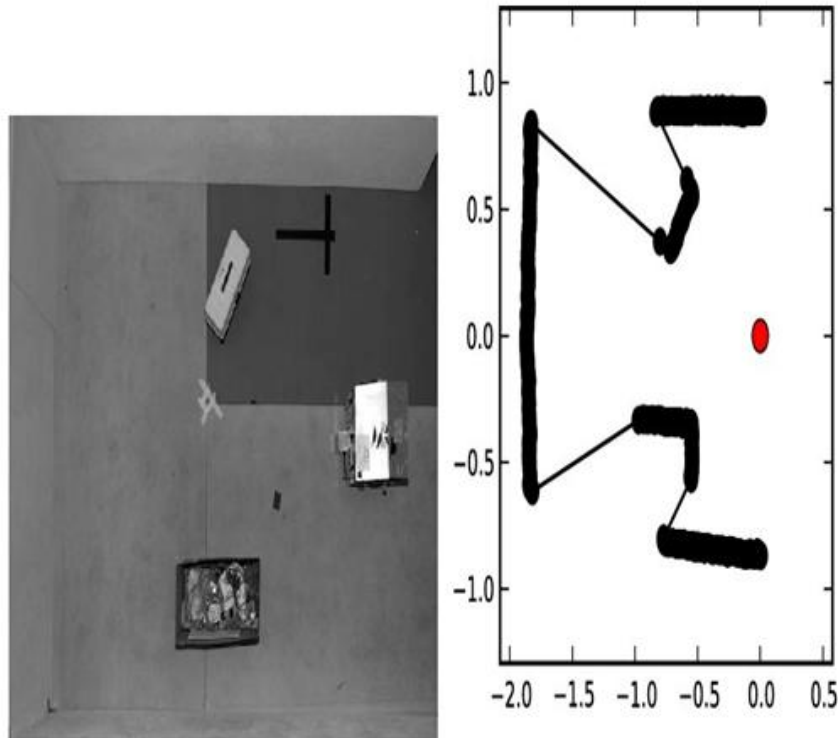
Fig.1: Obstacle Avoidance Setup and the Resultant Grid Map with the Collision Free
