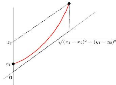
Figure 2.2: The cartesian coordinate for the catenary plane.
