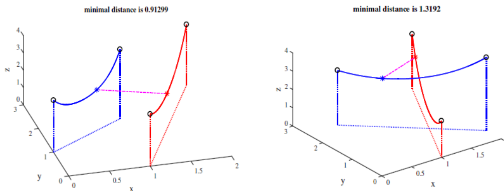
Figure 3.1: The minimal distance between two catenaries in two cases: the catenaries projected onto the (x, y) -plane have interjection point (left subfigure) and have no interjection point (right subfigure). The data for the these two cases are listed in Table 3.1.
