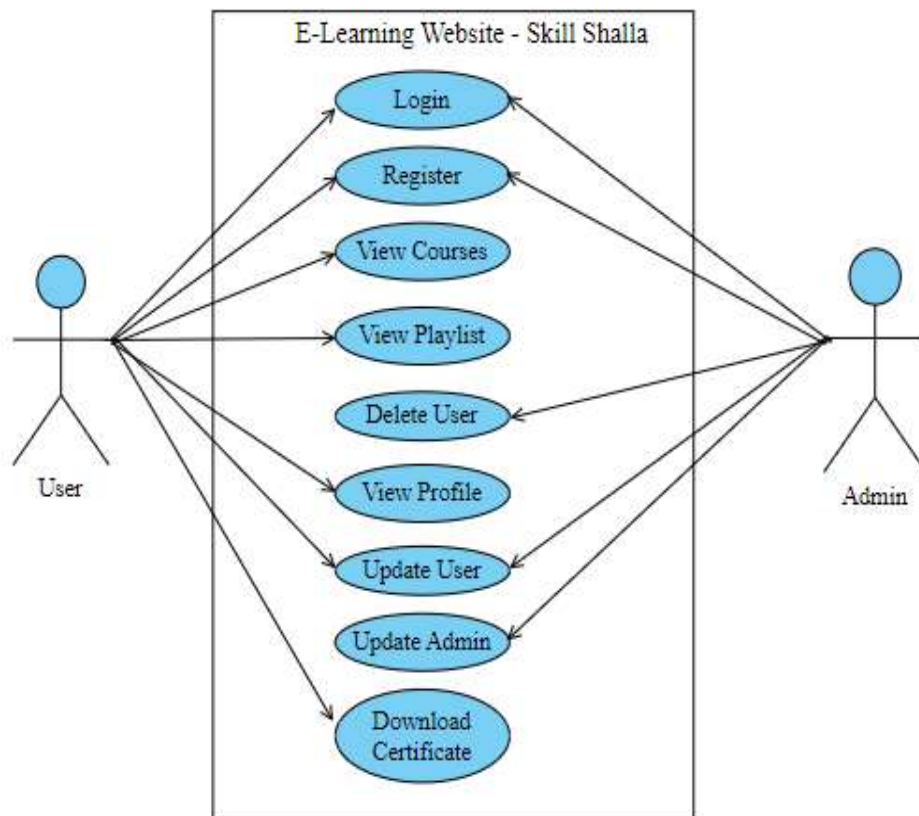
Fig 1.2 – Use Case Diagram
