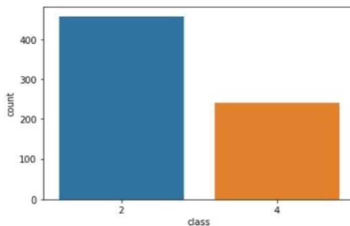
Figure 2. The number of benign and malignant cases; 2- benign 4-malignant.
