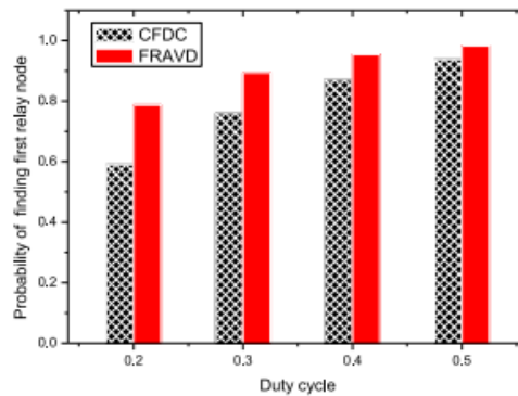
Fig. 5. Probability of finding first relay node at different duty cycles in CFDC and FRAVD.
