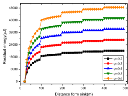
Fig. 2. Residual energy with different distances from sink.
