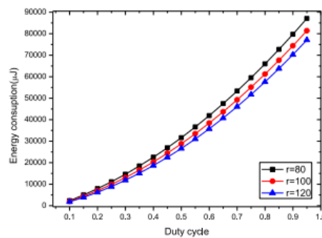
Fig. 1. Energy consumption with different duty cycles
