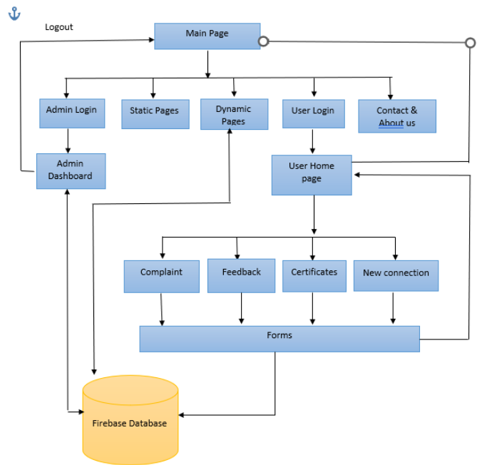
Figure 2. Flowchart
