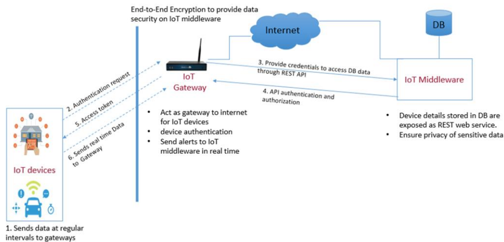
Figure 5: Proposed System Model.
