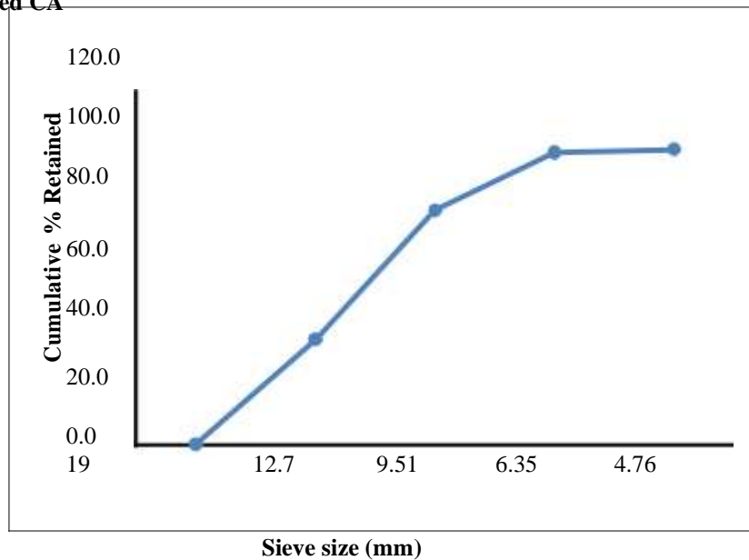
Figure 5. Gradation of Crushed Coarse Aggregates
