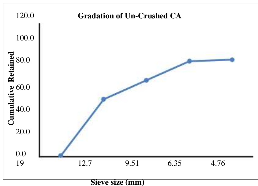
Figure 6. Gradation of Un-Crushed Coarse Aggregate
