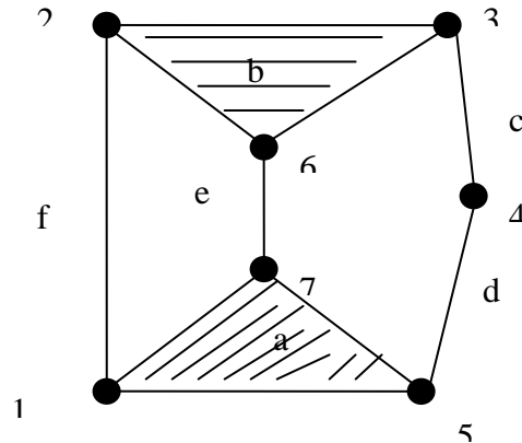
Fig.9: Six bar chain, single freedom
