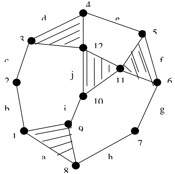
Fig.5: Ten bar chain, three freedom
