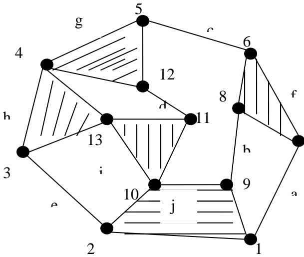
Fig.6: Ten bar chain, single freedom
