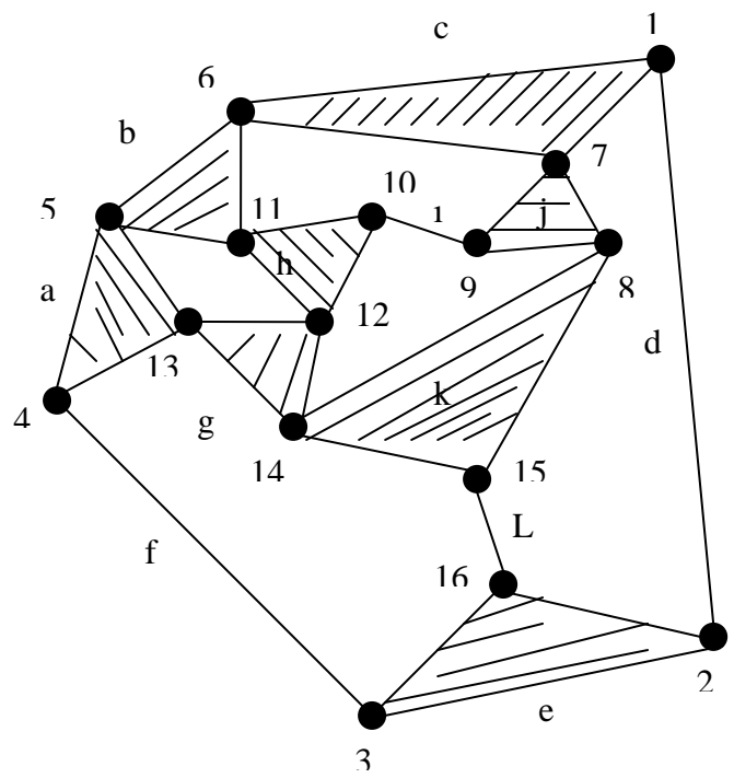
Fig.2: Twelve bar chain, single freedom
