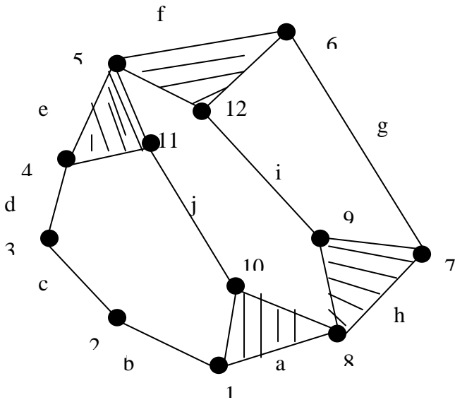
Fig.4: Ten bar chain, three freedom
