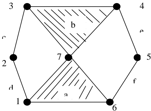
Fig.8: Six bar chain, single freedom
