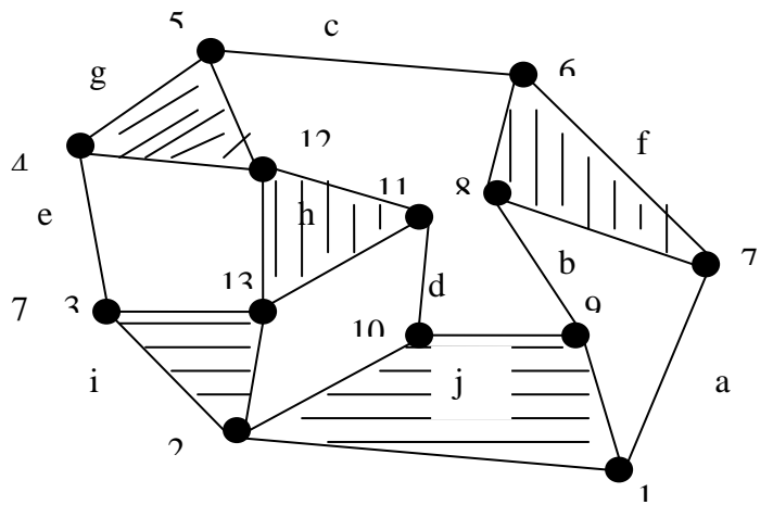
Fig.7: Ten bar chain, single freedom
