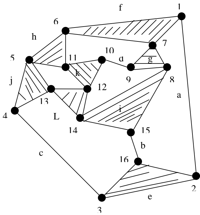
Fig.1: Twelve bar chain, single freedom
