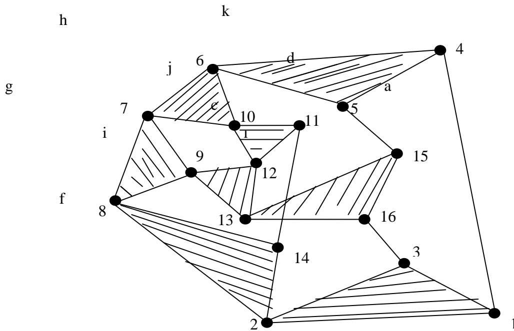
Fig.3: Twelve bar chain, single freedom
