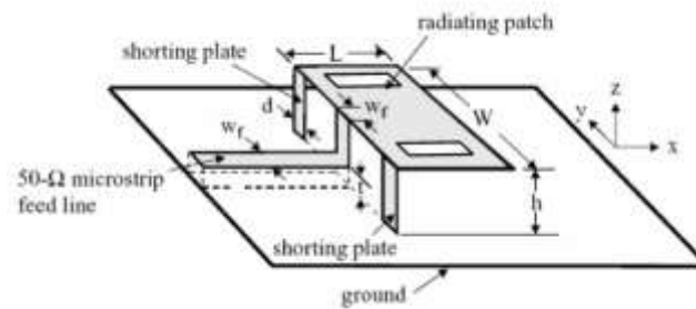
Figure 1(a) Microstrip line fed shorted patch antenna with vertical slots.
