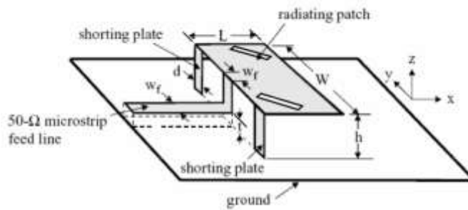
Figure 1(b) Microstrip line fed shorted patch antenna with inclined slots.
