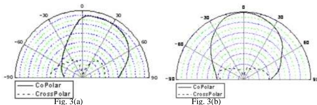
Figure 3 Radiation Pattern for Antenna with Vertical and Inclined slots
